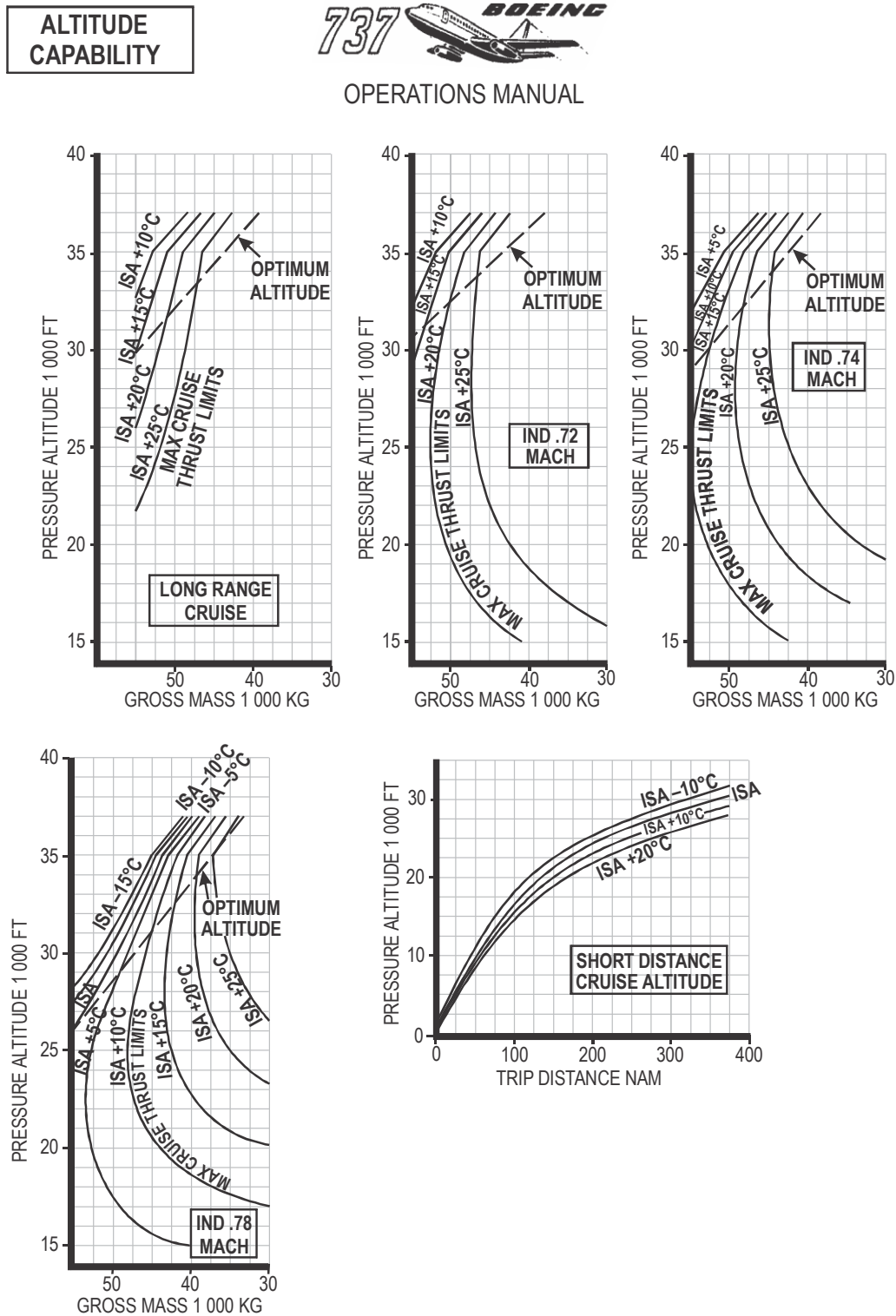
Figure F-3. Optimum flight level (for B737) as a function of take-off mass and temperature deviation from standard
