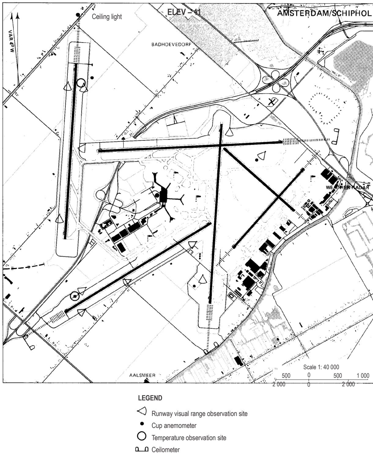
Figure B-3. Typical layout plan of meteorological instruments at an aerodrome
